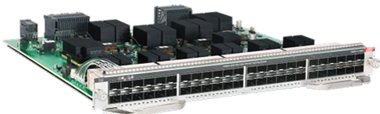
Figure 11. Cisco Catalyst 9400 Series 48-port 10 Gigabit Ethernet (SFP+) Line Card (C9400-LC-48XS)
