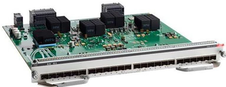
Figure 12. Cisco Catalyst 9400 Series 24-port 10 Gigabit Ethernet (SFP+) Line Card (C9400-LC-24XS)
