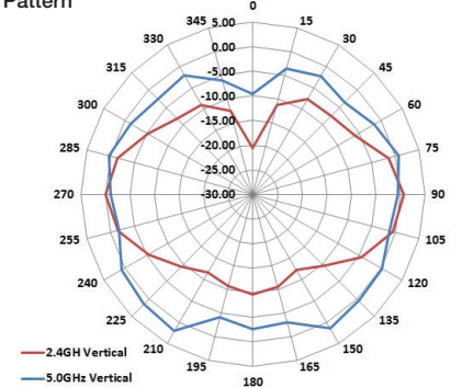
E-Plane Pattern
