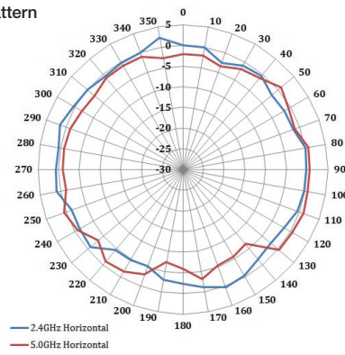
E-Plane Pattern
