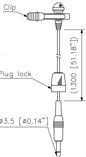
Lavalier Microphone
